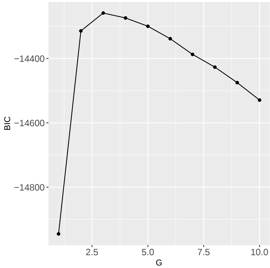
Figure 3: Bayesian Information Criterion (BIC) for the independent Poisson mixture model.
