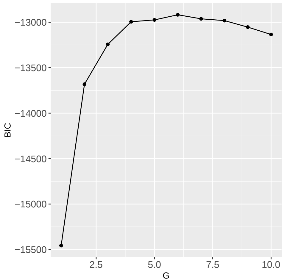
Figure 6: Bayesian Information Criterion (BIC) for the independent Poisson mixture model with the selected variables.
