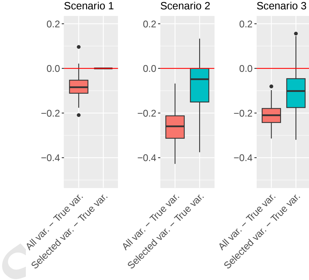
Figure 4: Distribution of the ARI differences with the model with the true clustering variables, for the model with the selected variables and the model with all variables.
